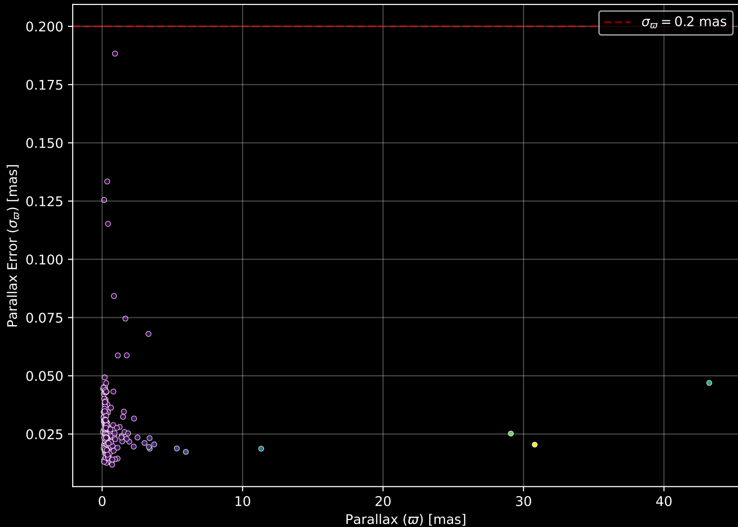
APOGEE DR17 Field: [203+00] Parallax Quality (n= 208)
