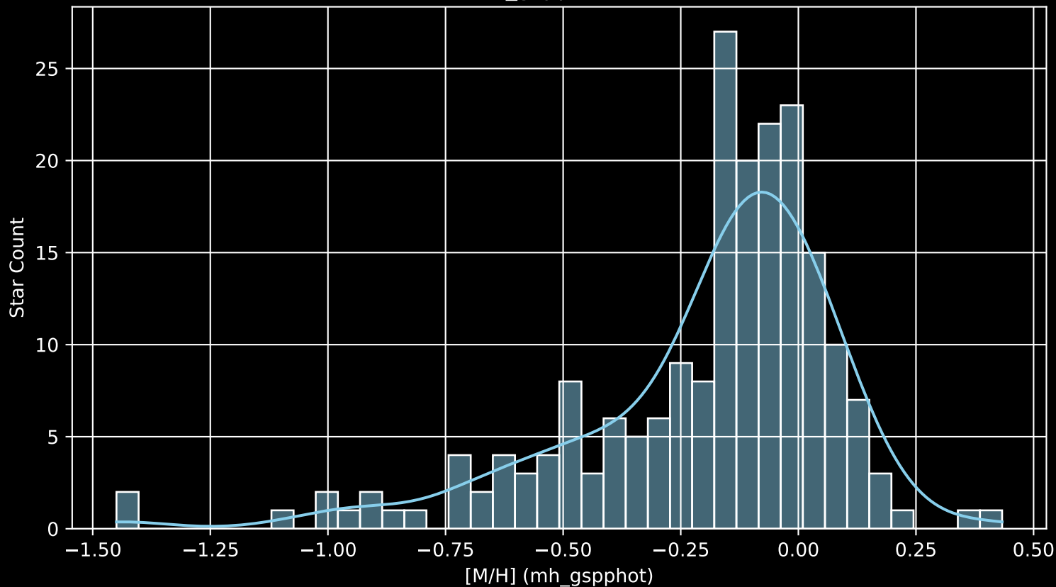
APOGEE DR17 Field: [203+00 [M/H] (mh_gspphot) (n= 202)
