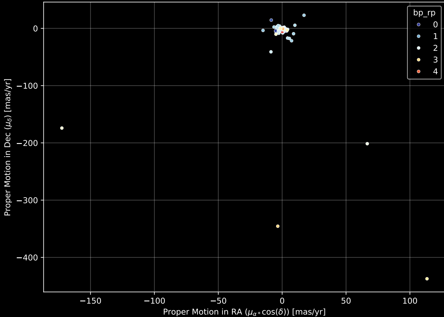
APOGEE DR17 Field: [203+00] Proper Motion Diagram (n= 208)
