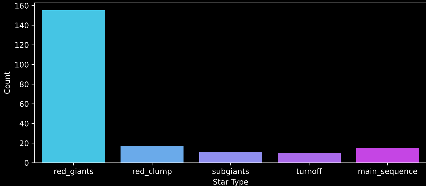
APOGEE DR17 Field: [203+00] Count plot of Star Type
