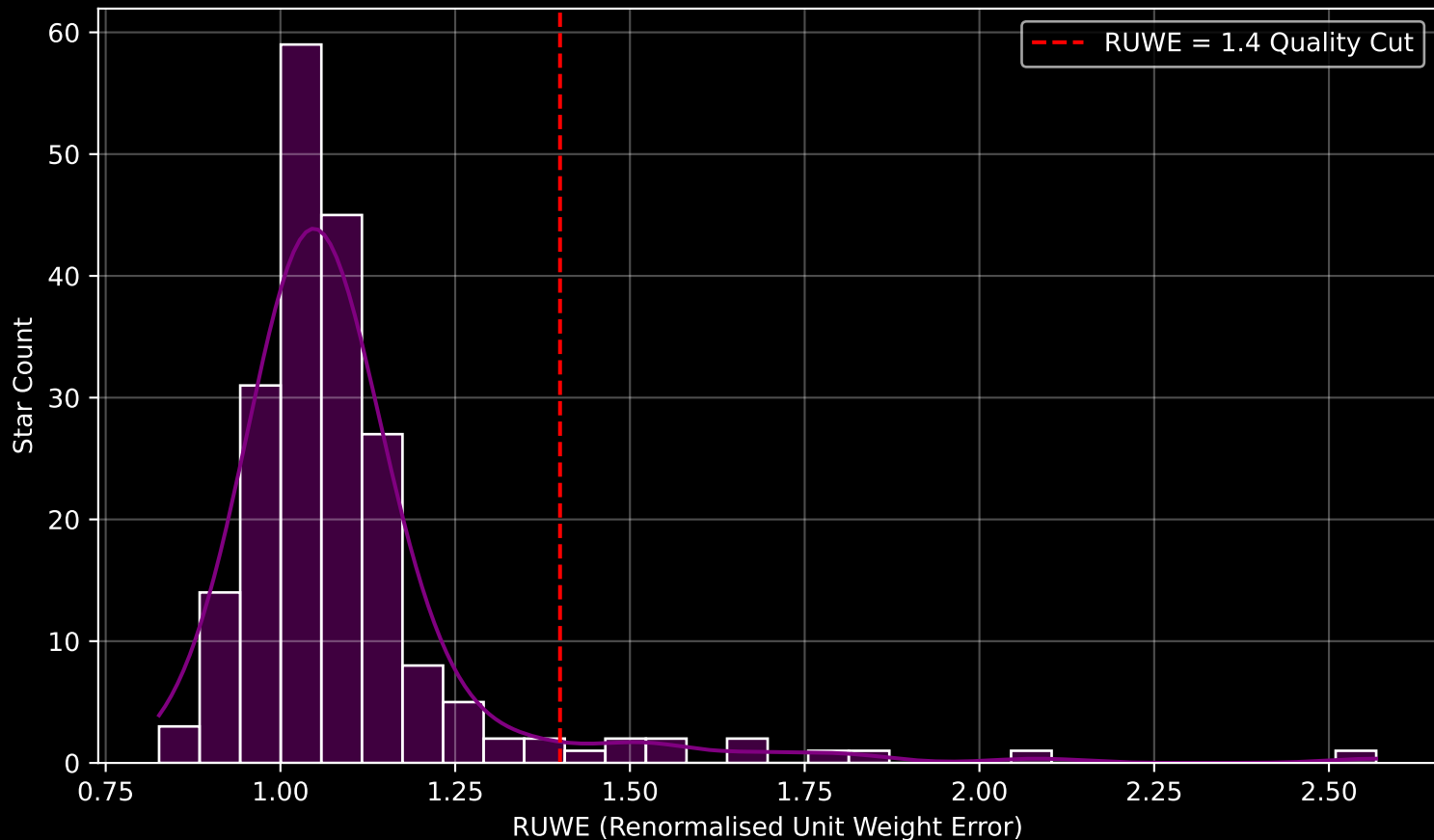
GAPOGEE DR17 Field [203+00] RUWE Distribution (n= 207)
